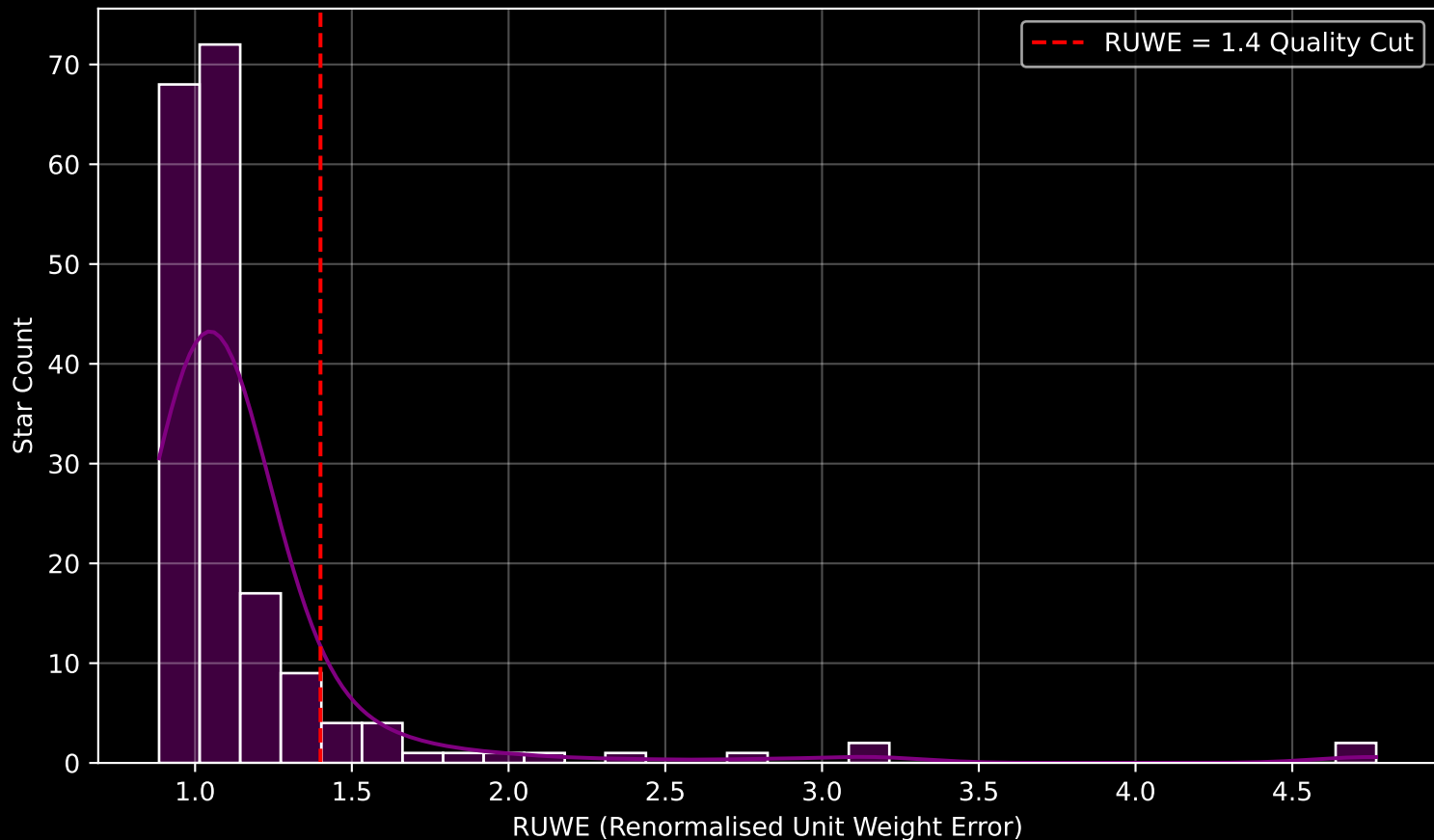
GAPOGEE DR17 Field [340+60] RUWE Distribution (n= 184)
