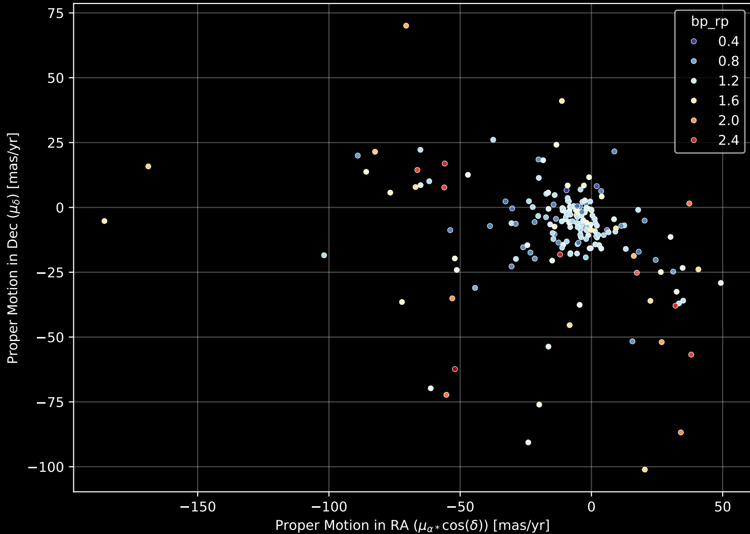
APOGEE DR17 Field: [340+60] Proper Motion Diagram (n= 189)
