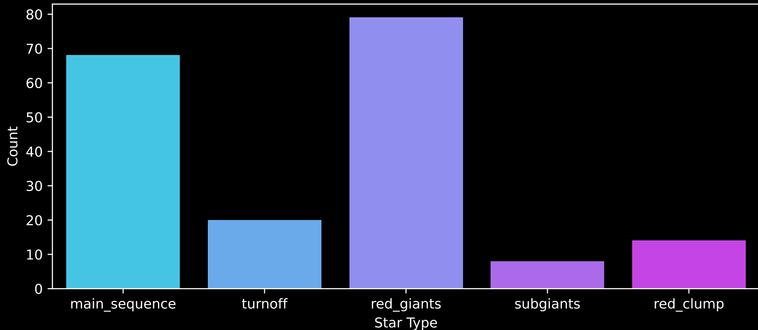
APOGEE DR17 Field: [340+60] Count plot of Star Type
