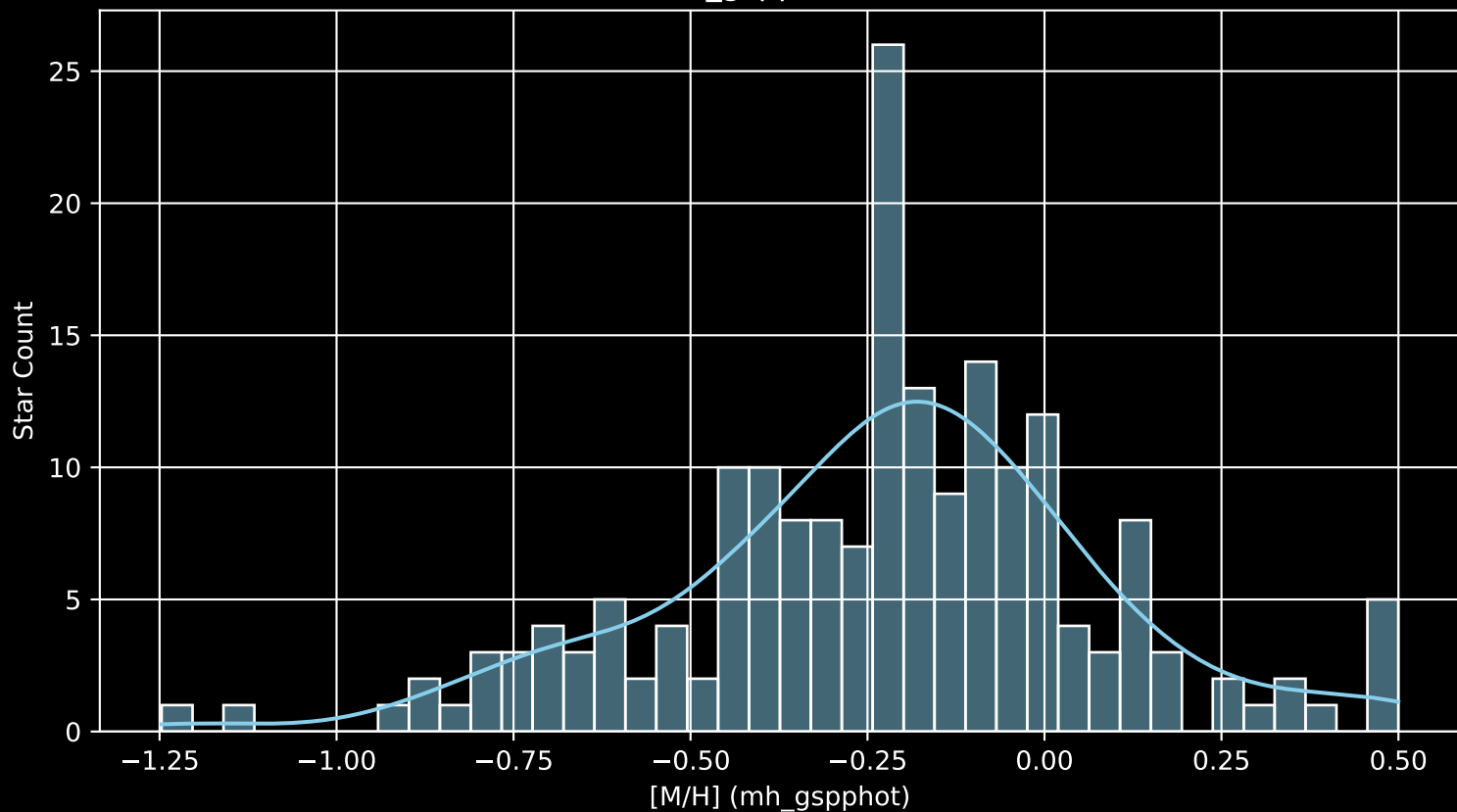
APOGEE DR17 Field: [340+60 [M/H] (mh_gspphot) (n= 188)
