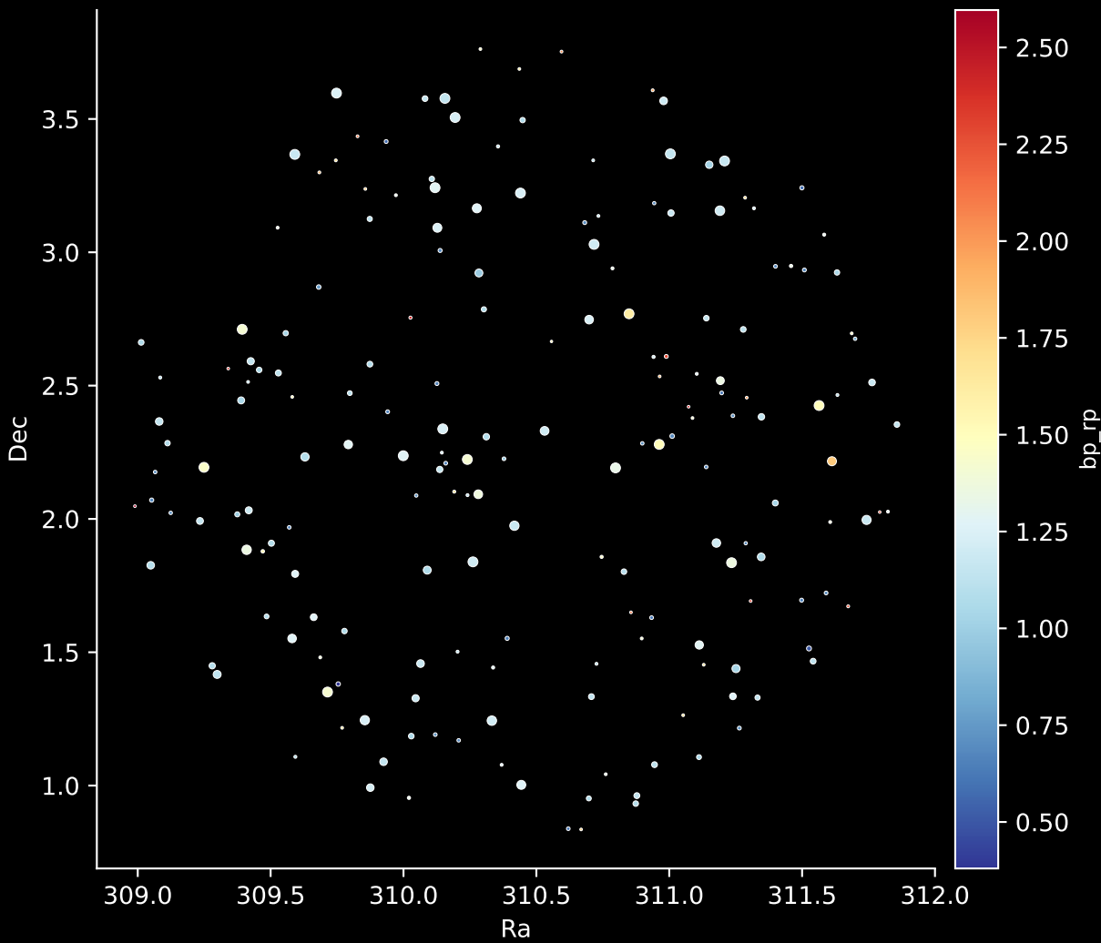
APOGEE DR17 Field: [340+60] Stars: 189
