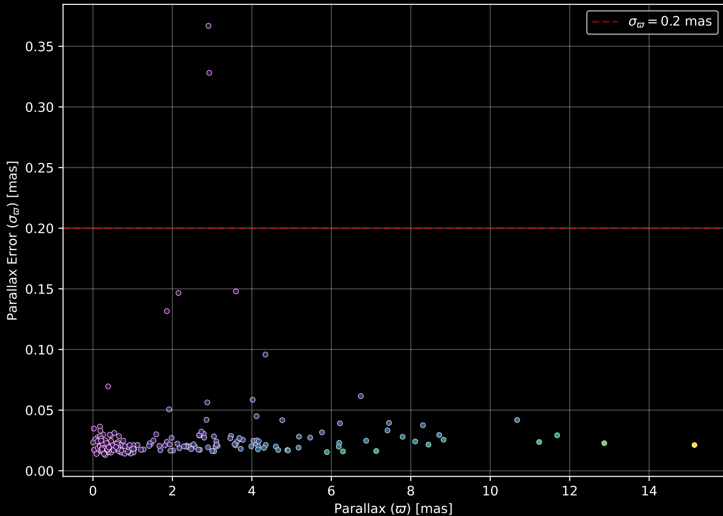
APOGEE DR17 Field: [340+60] Parallax Quality (n= 189)
