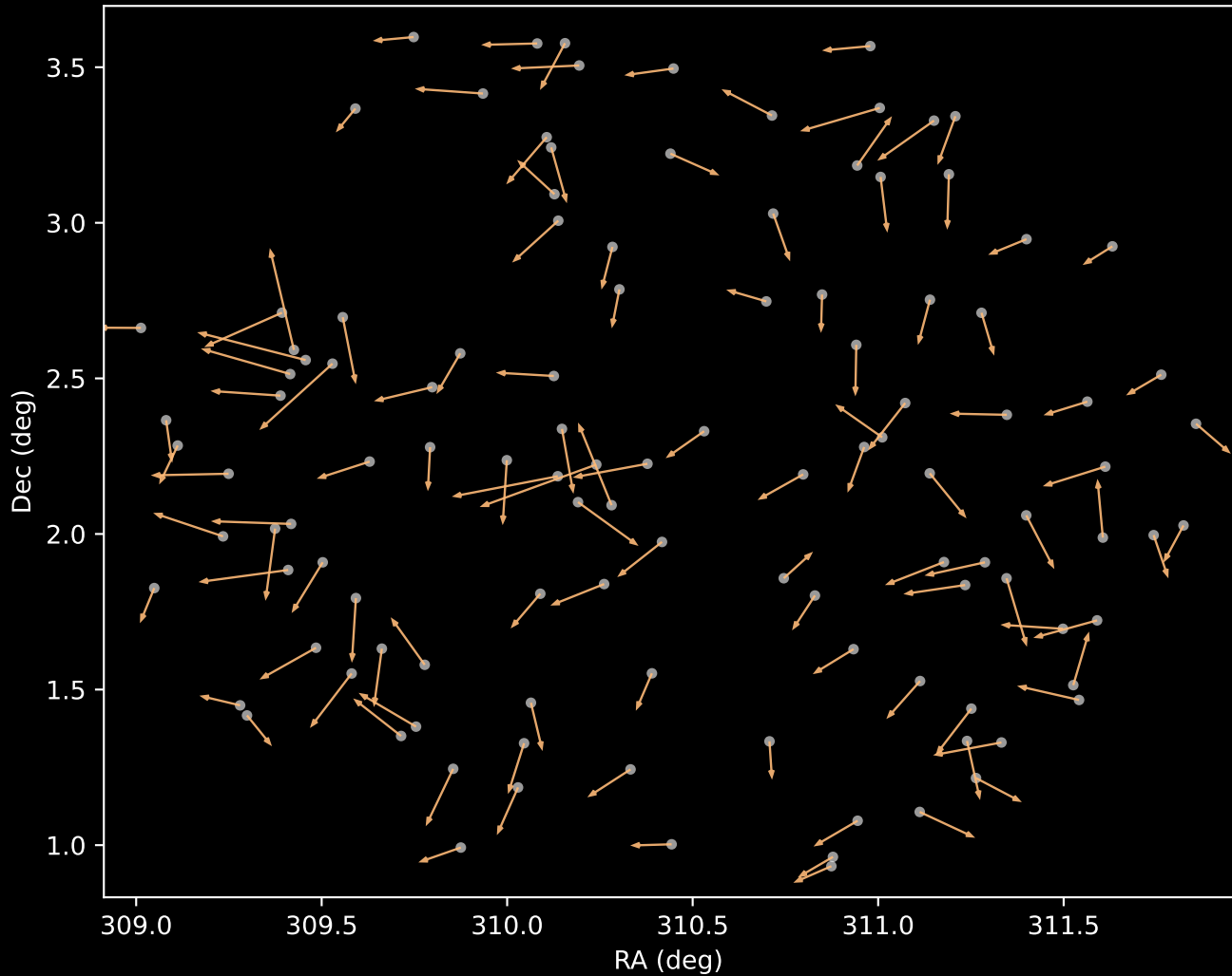
APOGEE DR17 Cluster 3 Proper Motion Vectors (n=115)
